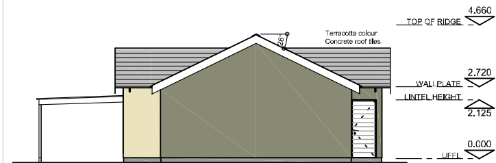
East Elevation
