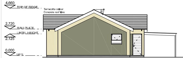
West Elevation
