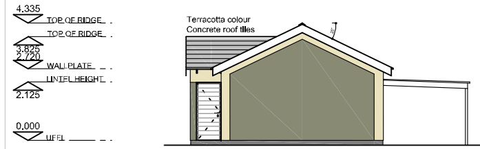
West Elevation
